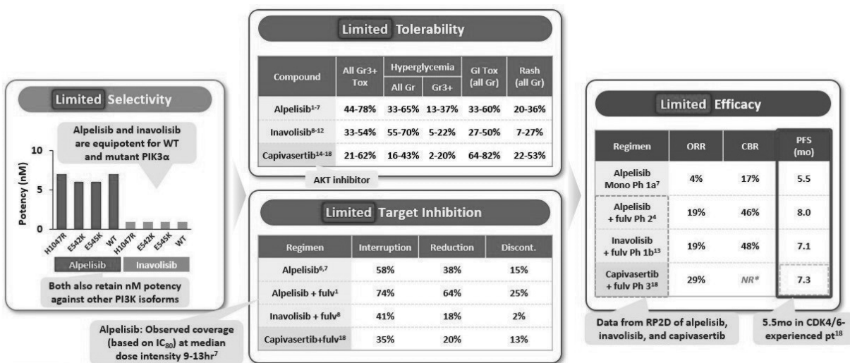
Figure 4: Existing inhibitors have limited therapeutic windows.
