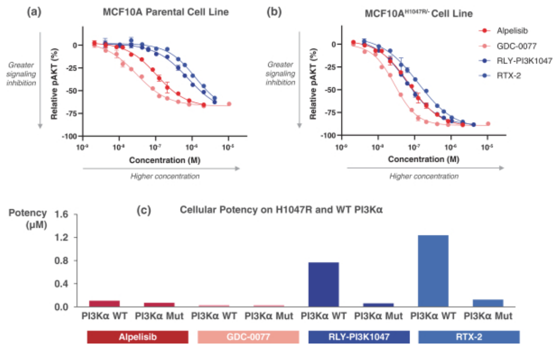
Figure 30: Compared to other clinical PI3K \alpha inhibitors (alpelisib and GDC-0077), Relay compounds more potently inhibits pAKT in cells expressing H1047R mutant PI3K \alpha compared to cells expressing wild-type PI3K \alpha .
