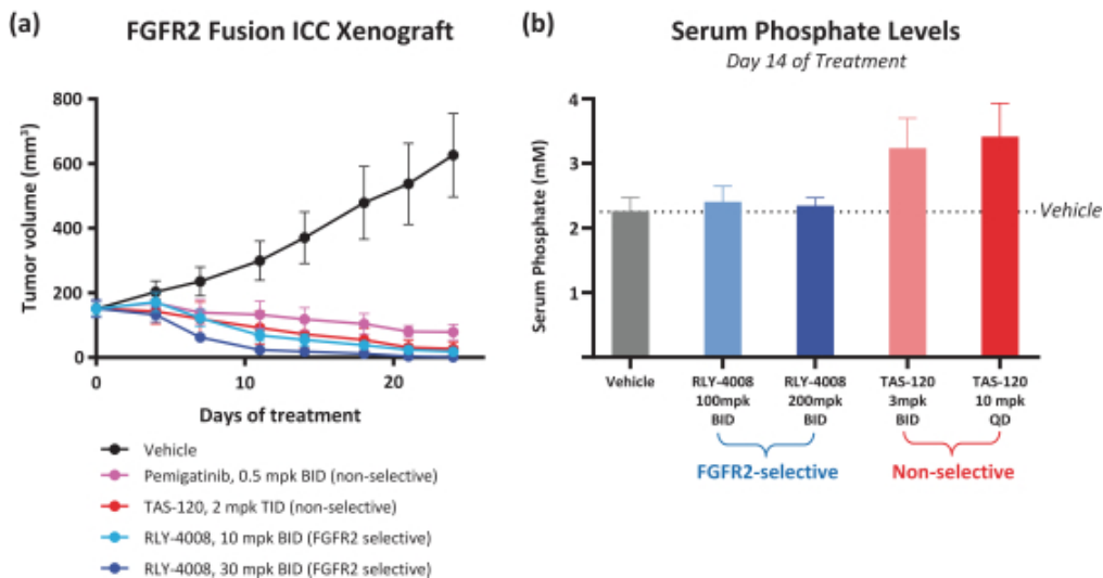
(a) Anti-tumor activity of RLY-4008 dosed twice daily (BID) by oral administration in an FGFR2 fusion-positive ICC PDX model. RLY-4008 induced dose-dependent regression when administered at 10 or 30 mpk BID. TAS-120 at 2 mpk TID (red) and pemigatinib at 0.5 mpk BID (pink) were dosed at levels selected to match their clinical exposures. Data points indicate mean tumor volume (n=6 per group) and error bars represent standard error of the mean. All treatment groups are statistically significant when compared to vehicle with p<0.001 as determined by two-sided t-test. (b) Serum phosphate measurements in rats dosed twice daily with RLY-4008 (blue) or TAS-120 (red) by oral administration. Doses of RLY-4008 (100 and 200 mpk BID) resulting in exposures leading to tumor regression in our FGFR2 gene fusion ICC PDX model do not cause significant hyperphosphatemia. Doses of TAS-120 (3 mpk BID and 10 mpk QD) selected to match human exposures in clinical studies cause significant hyperphosphatemia. Data indicate the mean serum phosphate level (n=5 per group), and error bars represent standard deviation. TAS-120 treatment groups are statistically significant when compared to vehicle with p<0.01 as determined by one-way ANOVA.
